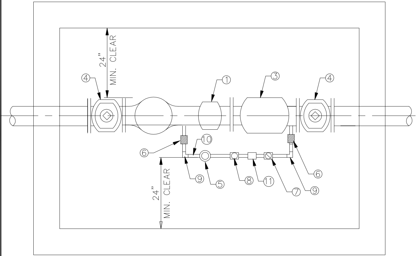
PLAN VIEW
